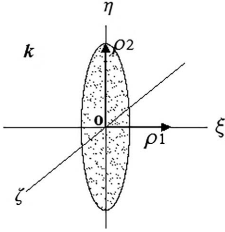
FIG. 4. The radius \rho_2 = c\tau of the expanding light-circle in the \eta - \xi plane (shaded area) is not the same as \rho_1 = c\tau of the light wavefront on the \xi -axis in the direction of motion v , because the respective times \tau are not the same since time depends upon position \xi in system K under Lorentz transformation from system K .
